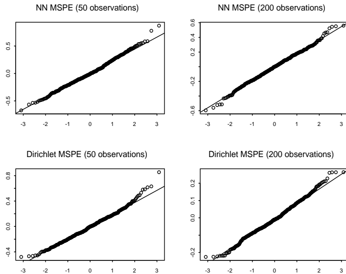
Figure 2: Quantile-quantile plots of the MSPE for \mu_1 (Gaussian mixture)
