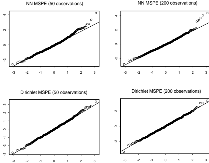
Figure 1: Quantile-quantile plots of the MSPE for \sigma_2 (Gaussian density)
